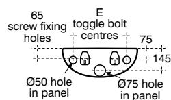
back view showing fixing in panels
