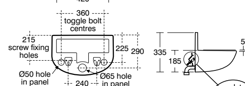
back view showing fixing in panels
